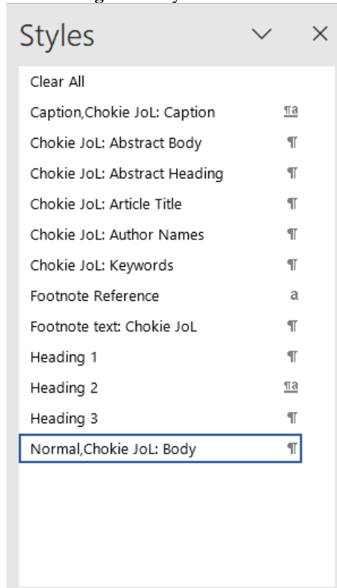
Figure 2: Styles window.
